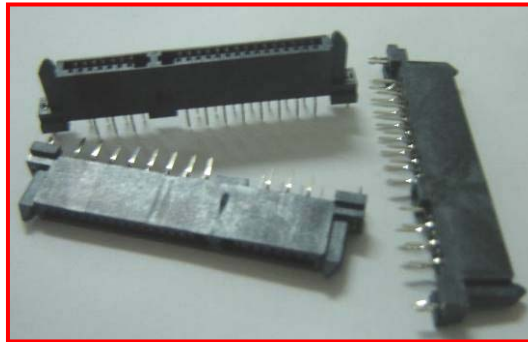
SATA 22P F (DIP TYPE)
